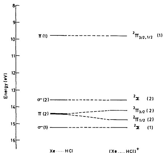
FIG. 2. Molecular orbital scheme for Xe...HCl in the ground and the ionic states.
