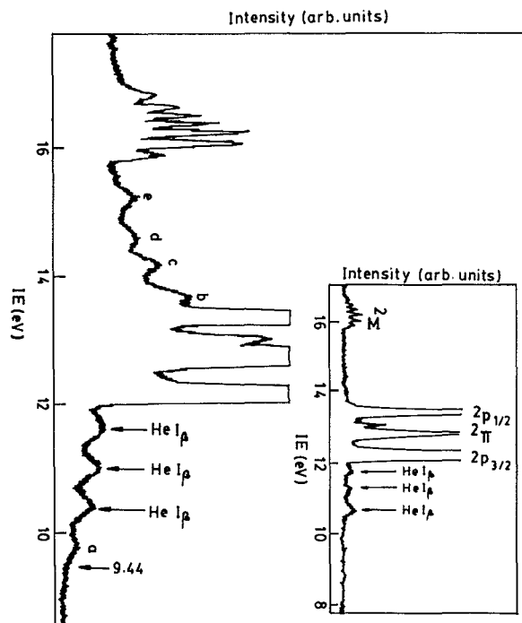
FIG. 1. UVPE spectrum of a Xe + HCl mixture recorded at a high stagnation pressure. Features a through e are due to the van der Waals molecule. He I B features are also indicated. Inset shows the spectrum of Xe + HCl at a low stagnation pressure.
