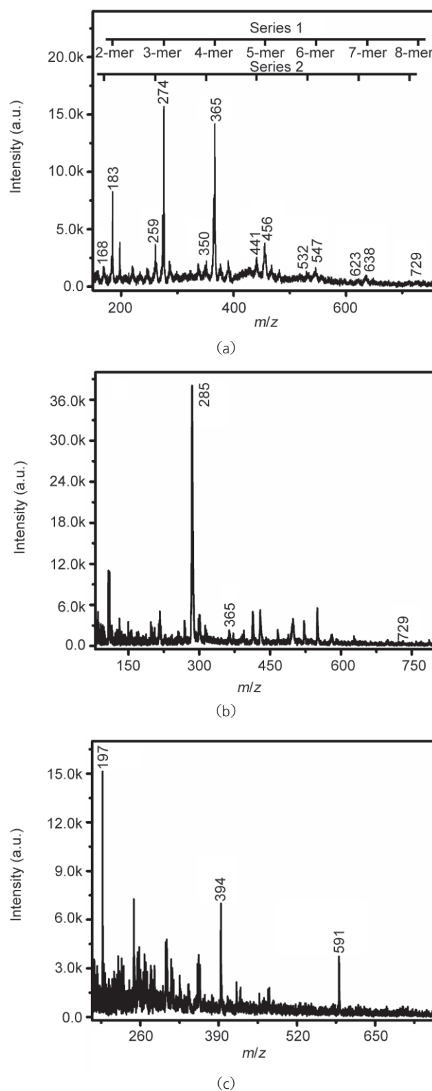
Figure 6 (a) LDI MS of the Au/oligoaniline seed taken in the positive mode. The two series of oligomeric peaks are indicated. Peaks in series 2 occur at m/z 15 lower than the corresponding peaks in series 1. (b) and (c) are the LDI MS of the mesoflower taken in positive and negative modes, respectively. The peak at m/z 285 in (b) due to the cetyltrimethylammonium ion is enhanced due to its high sensitivity
