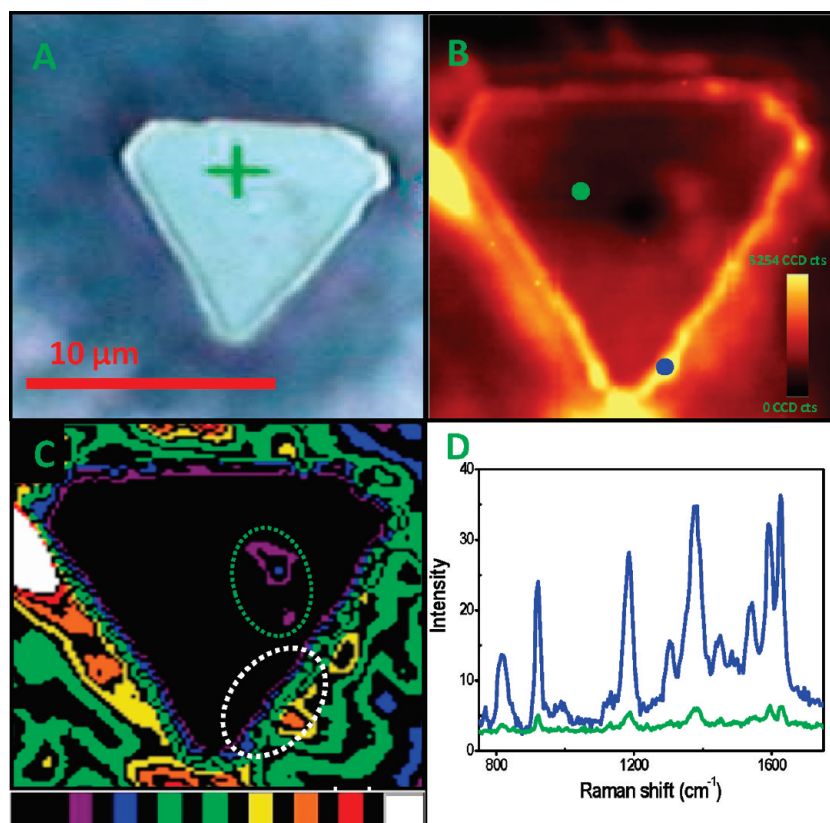
Figure 6. (A) Optical image (under white light illumination) of the Au@MSA SL triangle. (B) Raman image of the same crystal (at 514.5 nm excitation) collected from an area of 12\mu\text{m} \times 12\mu\text{m} using the intensities of CV features in the 200 to 2000\text{ cm}^{-1} window. The concentration of CV exposed was 10^{-5}\text{ M} . (C) Color coded Raman image of Au@MSA SL triangle shown in part A. The intensity is in the order: green > blue > pink > black. (D) Raman spectra collected from the edge (blue) and surface (green) of the crystal shown in part B.
