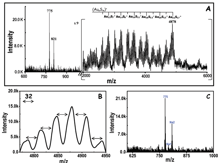
FIGURE 2. (A) MALDI-TOF MS of Au 22 in the positive mode showing the presence of Au 22 S 17 . A group of peaks is separated by m/z 197, due to gold, between the adjacent major peaks. (B) Expanded view of the last few sets of peaks in part A, showing a separation of m/z 32 due to sulfur. (C) Expanded view of the mass spectrum collected in the lower mass region in part A, showing the presence of a H 2 TPPOAS − ligand ( m/z 775) and one and two sodium pickups (marked Na1 and Na2).
