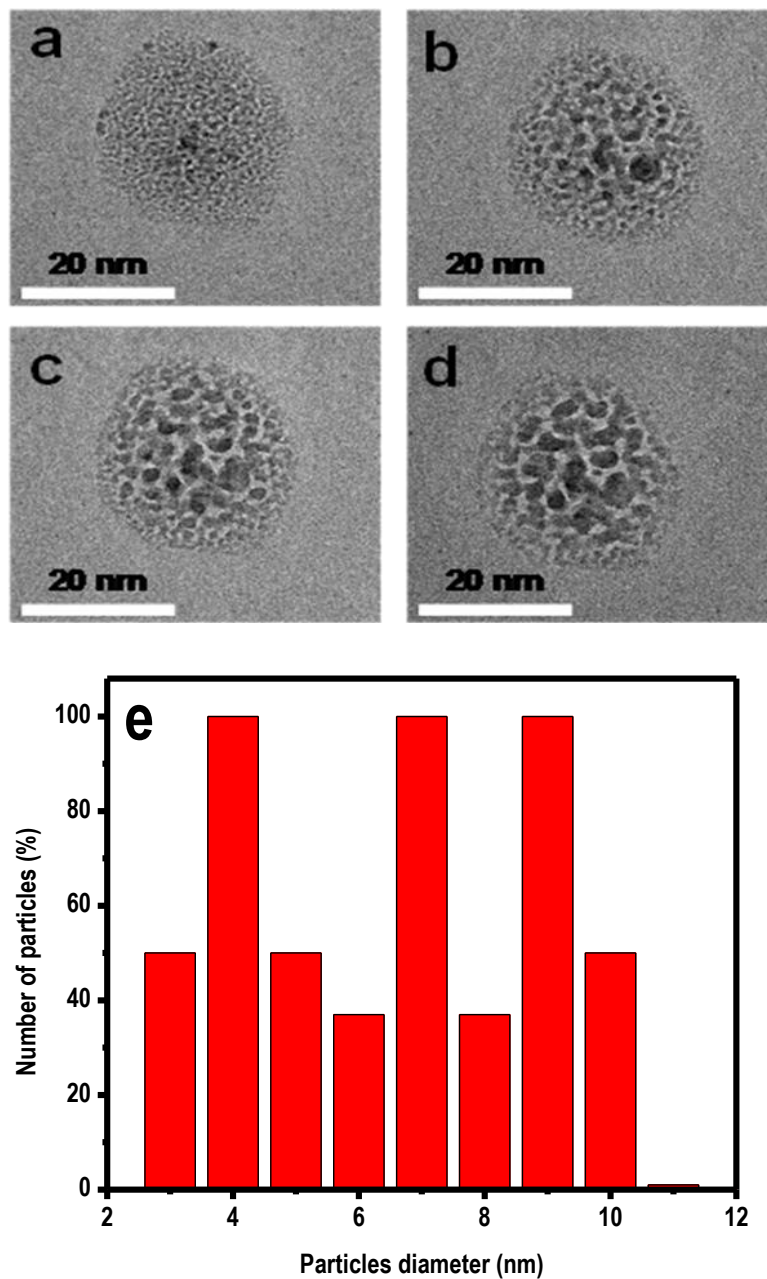
Fig S4. TEM image of phase transferred Ag QC @MSA cluster aggregates upon continuous electron beam irradiation. The same regions of the grid are shown in images a, b, c and d. Image 'a' is at the start of the irradiation showing small clusters, image 'b' is after 30 sec. In 'c' the irradiation time was 60 sec. It was 90 sec in 'd'. Diagram 'e' is the particle size distribution corresponding to the TEM image 'd'. Various size distributions from 3 to 11.5 nm are due to Ag QC @MSA cluster aggregates, upon electron beam irradiation.
