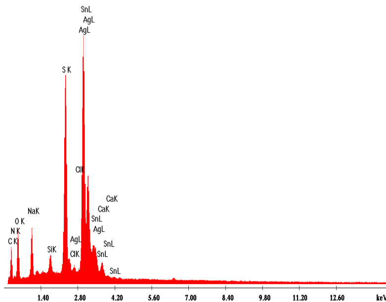
Fig S8. A) SEM and EDAX images of the cluster. EDAX maps using C K α , Ag L α , and S K α are shown. B) EDAX spectrum of AgQC@MSA cluster.
