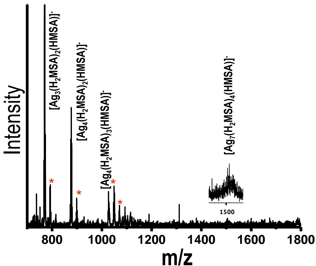
Fig S5. ESI MS of the Ag QC @MSA cluster collected in the negative mode. Peaks with * show the Na adducts of the preceding formula. These appear to be decomposition products.
