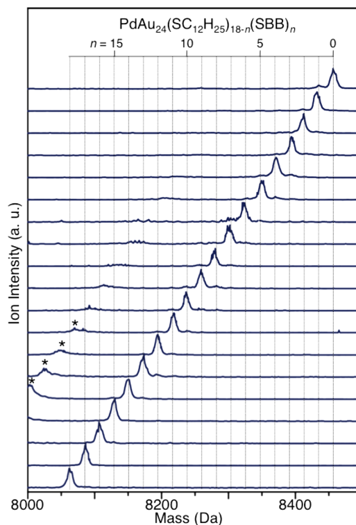
Figure 2. Negative-ion MALDI mass spectra of each cluster of composition \text{PdAu}_{24}(\text{SC}_{12}\text{H}_{25})_{18-n}(\text{SBB})_n ( n = 0\text{--}18 ), isolated in this work. The asterisks indicate laser-induced fragments.
