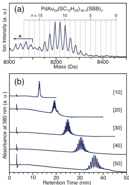
Figure 1. (a) Negative-ion MALDI mass spectrum of \text{PdAu}_{24}(\text{SC}_{12}\text{H}_{25})_{18-n}(\text{SBB})_n ( n = 6\text{--}16 ). The asterisk indicates laser-induced fragments. 35 (b) Chromatograms of \text{PdAu}_{24}(\text{SC}_{12}\text{H}_{25})_{18-n}(\text{SBB})_n ( n = 6\text{--}16 ) at each gradient program (see the text). The peak observed at 3.0 min was confirmed to be due to the solvent, THF.
