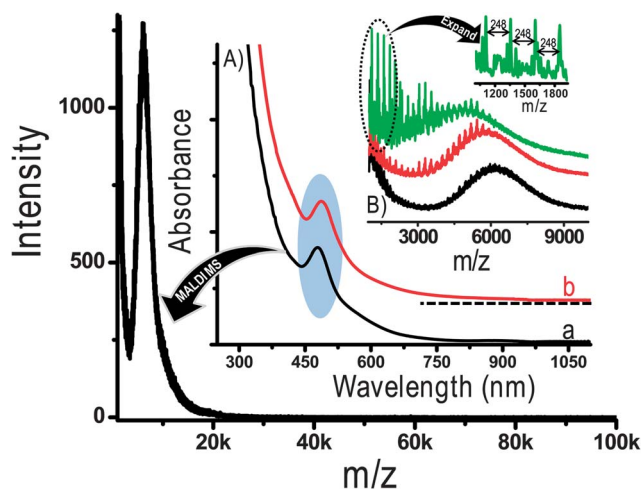
Fig. 4 MALDI MS of \text{Ag@MPG} in negative mode. (A) UV-vis absorption spectra of \text{Ag@MPG} (a) and \text{Ag}_{32}\text{SG}_{19} (b) clusters at pH 6.0. (B) Laser dependent MALDI MS spectra of the \text{Ag@MPG} cluster at near threshold intensity (black trace, \sim 1700 ) and at higher laser intensities (red and green traces). Inset of B show the expanded region of MALDI MS at high laser intensity ( \sim 3500 ).
