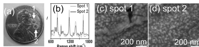
Figure 1. a) Two AgNP-containing spots created on a penny coin by electrolytic spray ionization deposition under ambient conditions. The top spot was created before drop casting a crystal violet sample ("NP-below") while the lower spot was created on top of a layer of crystal violet ("NP-on-top"). 10 Monolayers (ML) of silver ions were landed to create both spots, which showed similar morphology (c, d) and enhanced Raman signals (b).
