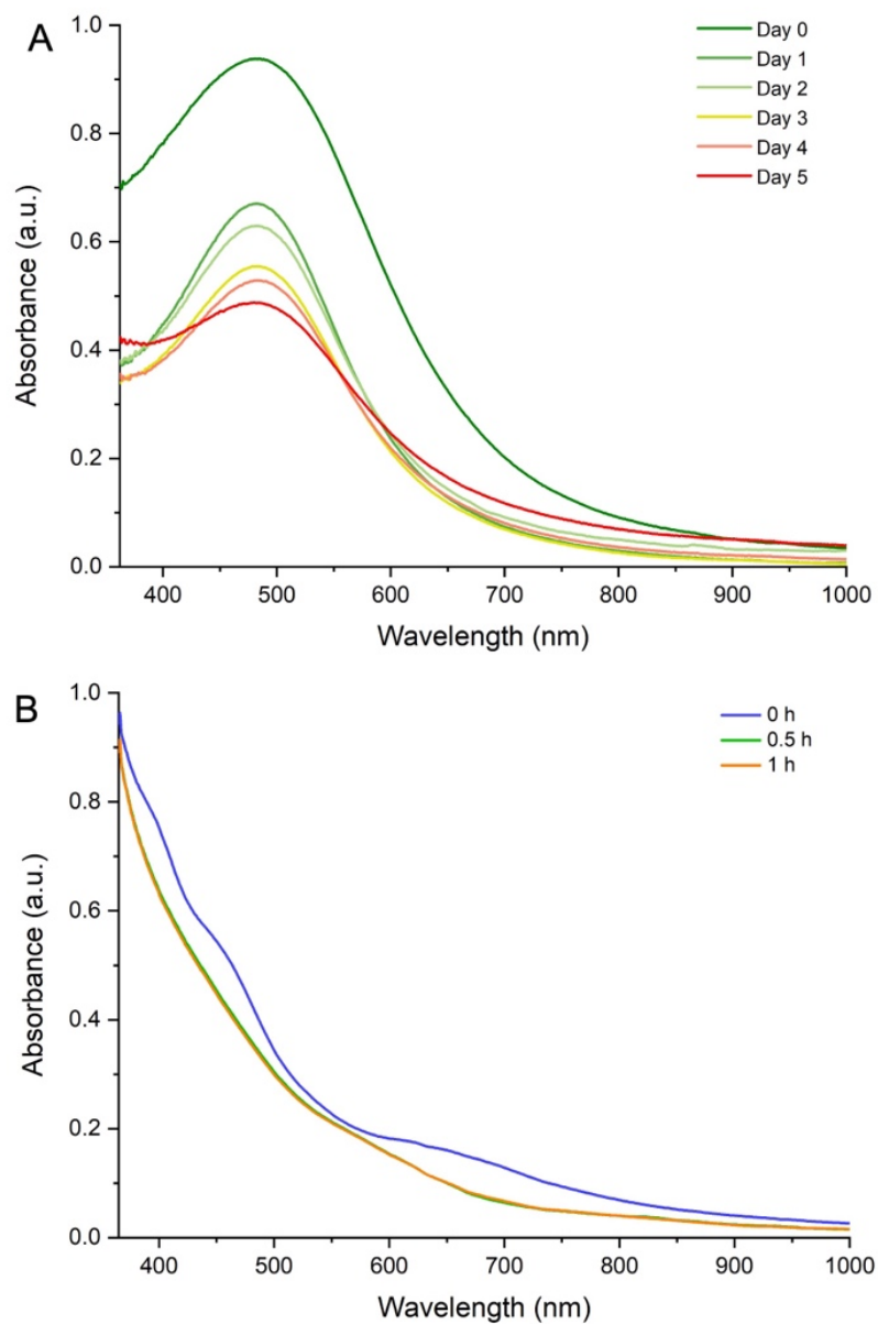
Fig. S13 Optical absorption spectra of the (A) parent polydispersed Ag@PET NPs, and (B) [Au 25 (PET) 18 ] - NC, showing degradation over time when heated to 45°C in toluene with a constant stirring at 250 RPM.
