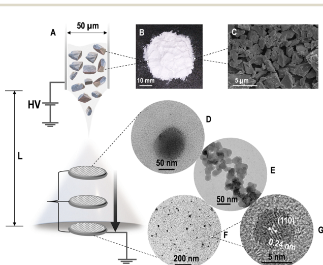
Fig. 1 The disintegration process of natural quartz particles in charged water microdroplets. Schematic diagram showing the different components of the home-built electrospray set-up with (A) a fused silica capillary of inner diameter 50\ \mu\text{m} , (B) an optical image of the ground quartz powder, and (C) field emission scanning electron microscopy (FESEM) of the separated quartz particles revealing the size range of 5\text{--}10\ \mu\text{m} . Transmission electron microscopic (TEM) images of these particles after electrospray deposition at an applied potential of 3.5\ \text{kV} , with varying tip-to-substrate distances of (D) 1.5\ \text{cm} , (E) 2.0\ \text{cm} , and (F) 2.5\ \text{cm} , demonstrating different stages of fragmentation. (G) High-resolution TEM (HRTEM) image showing the (110) plane of quartz.
