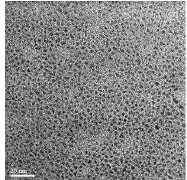
MoS 2 Nanoparticles
